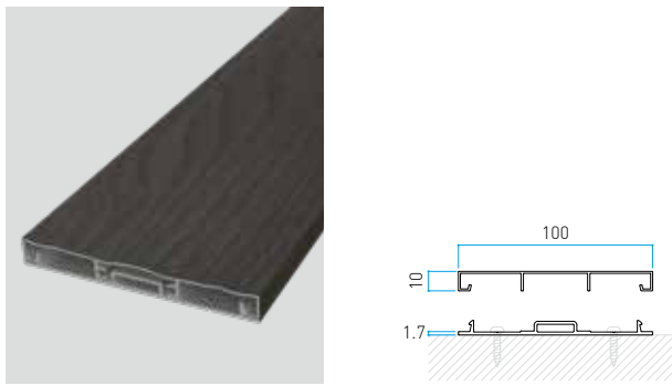
Size in mm 100x12xL4000 Real t: 1.0 mm
