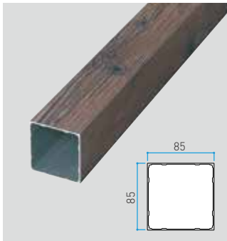
SLIT 85 Size in mm 85x85xL4000 t:1.3mm
