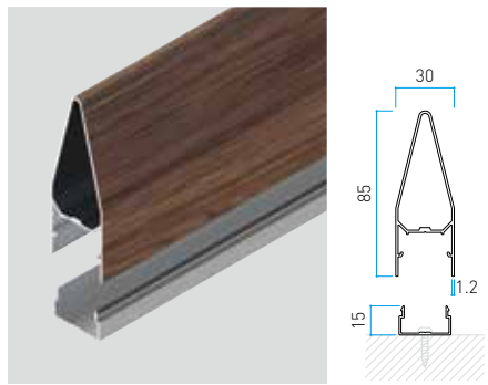
Size in mm 30x85xL4000 Katana t: 1.2 mm
