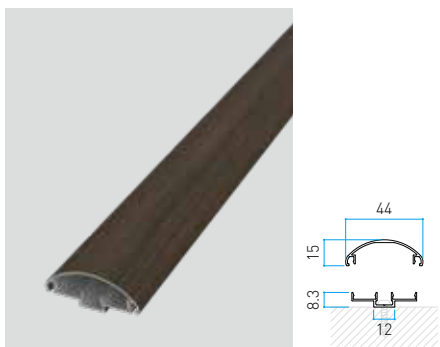
Size in mm 44x15xL3560 t: 1.0 mm
