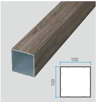
SLIT 100 Size in mm 100x100xL4000 t:1.5mm
