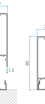
Size in mm 30x85xL4000 t:1.2mm
