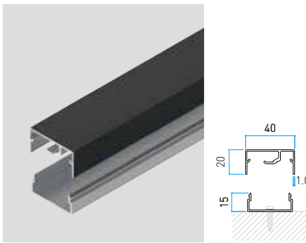
Size in mm 40x20xL4000 t: 1.0 mm
