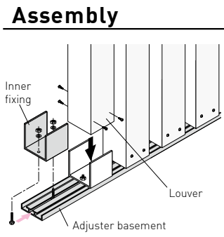
Turn & Slide system
