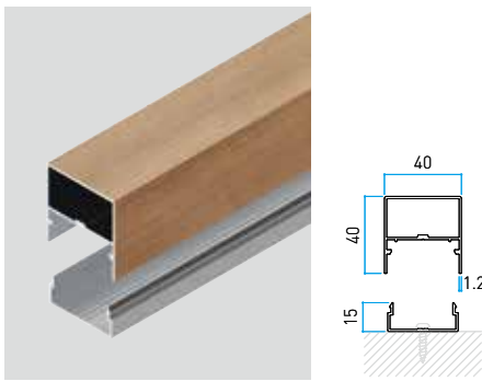
Size in mm 40x40xL4000 t: 1.2 mm
