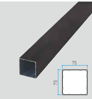
SLIT 75 Size in mm 75x75xL4000 t:1.2mm
