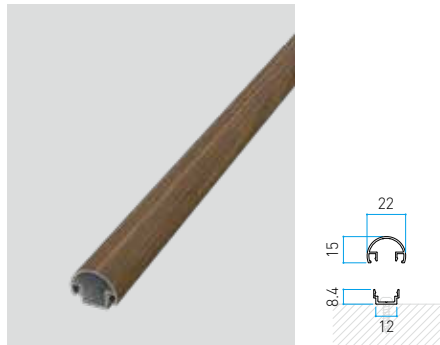
Size in mm 22x15xL3650 t: 1.0 mm
