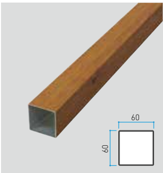
SLIT 60 Size in mm 60x60xL4000 t:1.2mm
