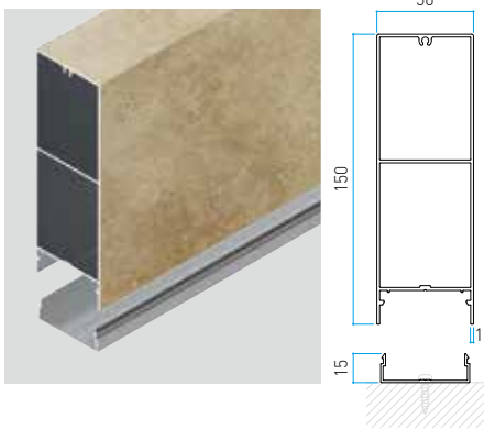
Size in mm 50x150xL3650 t: 1.5 mm
