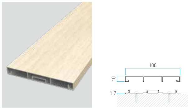
Size in mm 100x12xL4000 Flat t: 1.0 mm
