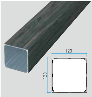
SLIT 120 Size in mm 120x120xL4000 t:1.6mm
