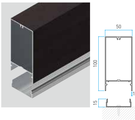
Size in mm 50x100xL3650 t: 1.3 mm
