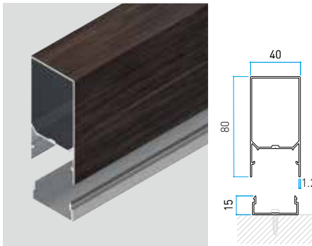
Size in mm 40x80xL4000 t: 1.2 mm
