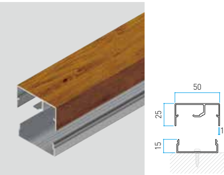
Size in mm 50x25xL4000 t: 1.2 mm
