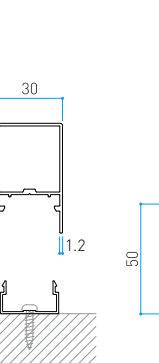
Size in mm 30x50xL4000 t:1.2mm
