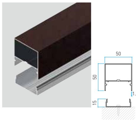
Size in mm 50x50xL3650 t: 1.2 mm
