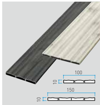
Board Real 100 & 150 Size in mm 100x10xL4000 t:1.0mm 150x10xL4000 t:1.0mm
