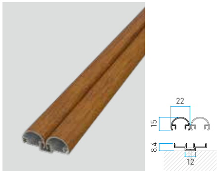
Size in mm 44.5x15xL3650 t: 1.0 mm
