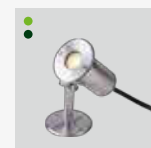
HHA-D10S W70xD101xH132mm 2.8W 3000K 160lm
