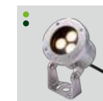
HHA-D11S W95xD106xH150mm 7.6W 3000K 570lm
