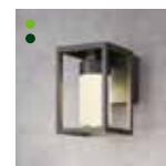
HBA-D25K W100xD146xH152mm 5.0W 3000K 150lm
