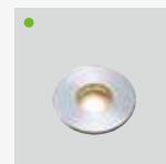
HHA-D06S W86xD86xH136mm 2.5W 3000K 111lm
