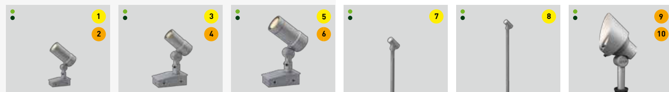
HBB-D32S W65xD105xH155mm 2.9W 3000K 200lm HBB-D34S W65xD124xH169mm 6.1W 3000K 560lm HBB-D36S W68xD140xH178mm 12.0W 3000K 950lm HBB-D30S W30xD60xH300mm 1.0W 3000K 1113lm HBB-D29S W30xD60xH500mm 1.0W 3000K 1113lm HBB-D17S W86xD119xH153mm 2.7W 3000K 207lm
