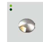
HHA-D13S W55xD55xH111mm 2.6W 3000K 10lm
