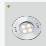
HHA-D07S W135xD135xH123mm 9.0W 3000K 500lm
