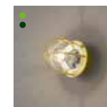
HBF-D28B W120xD120xH169mm 4.0W 2700K 224lm
