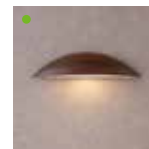
HBG-D08P W404xD97xH95mm 4.5W 2900K 90lm
